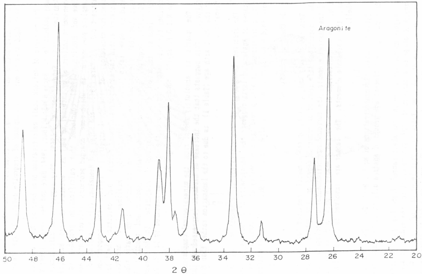
Figure 2: X-Ray diffraction pattern for mineralogical composition of Anadara diluvii
